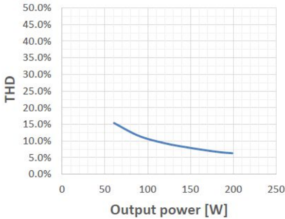
OT 240 2DIM NFC IP67 Typical THD vs Load
